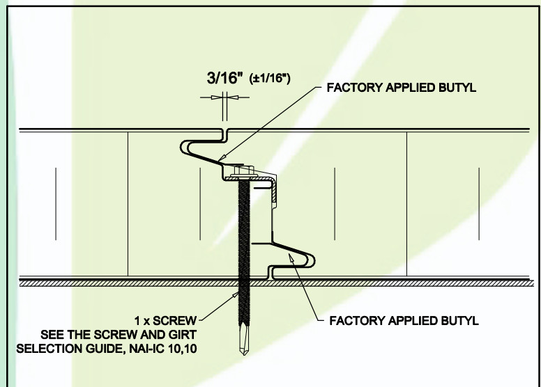
Figure 4.1: Joining Panels
